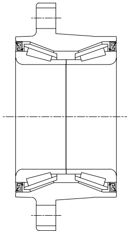
Tapered roller bearing (2 rows + 1 flange)
