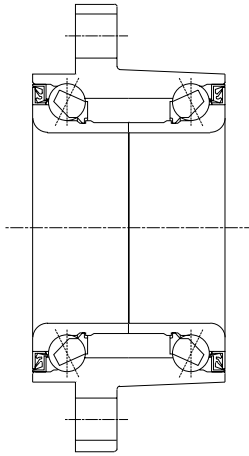
Angular contact ball bearing (2 rows + 1 flange)
