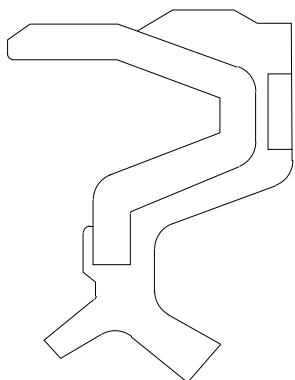
Two-lip seal reinforced
