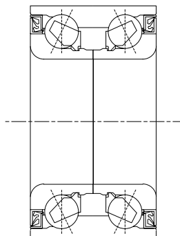
Angular contact ball bearing (2 rows)
