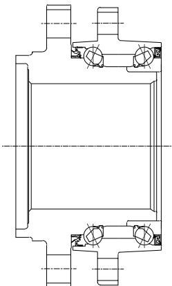
Angular contact ball bearing (2 rows + 2 flanges)
