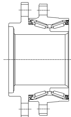
Tapered roller bearing (2 rows + 2 flanges)
